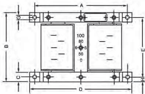
Vista Frontal
