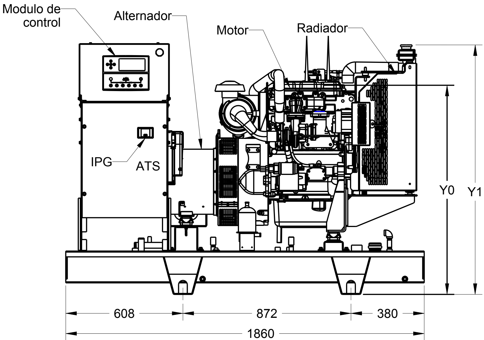
VISTA FRONTAL
