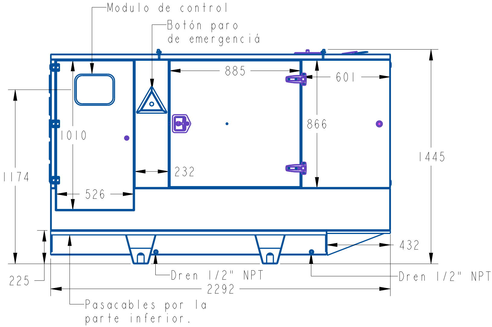
VISTA FRONTAL
